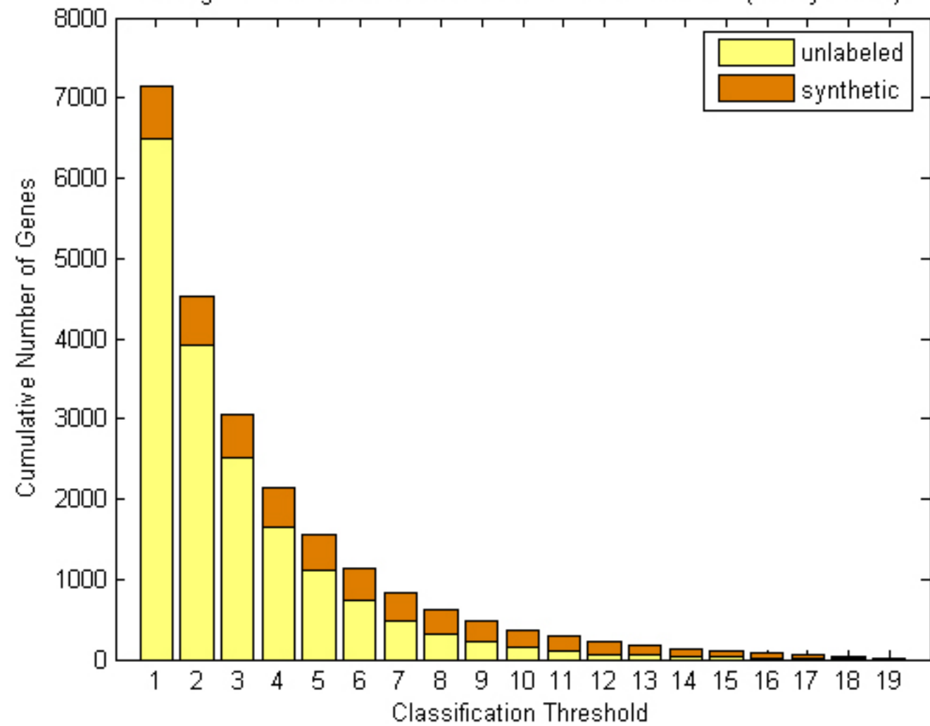
Average Genes Found at Each Classification Threshold (5% synthetic)
